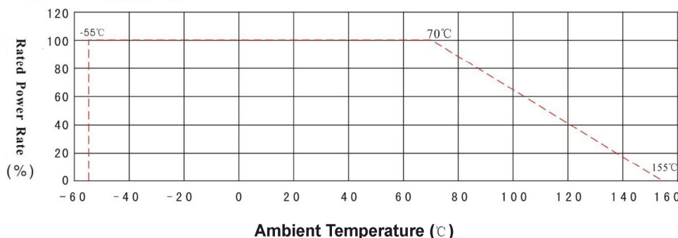
Rated Power Derating Curve
